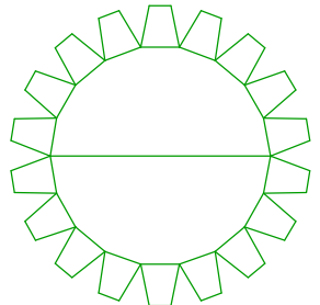
HALF CIRCULAR RE-INFORCEMENTS FOR MAIN BOILER. END AND CENTRE IF NEEDED
